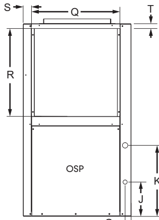
LEFT RETURN LEFT VIEW AIR COIL OPENING
