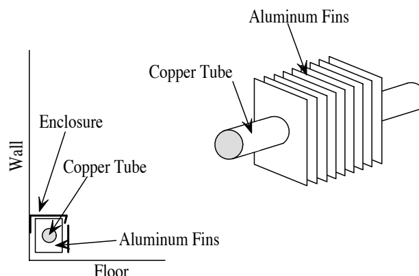
Figure 2-12: Baseboard Radiation
