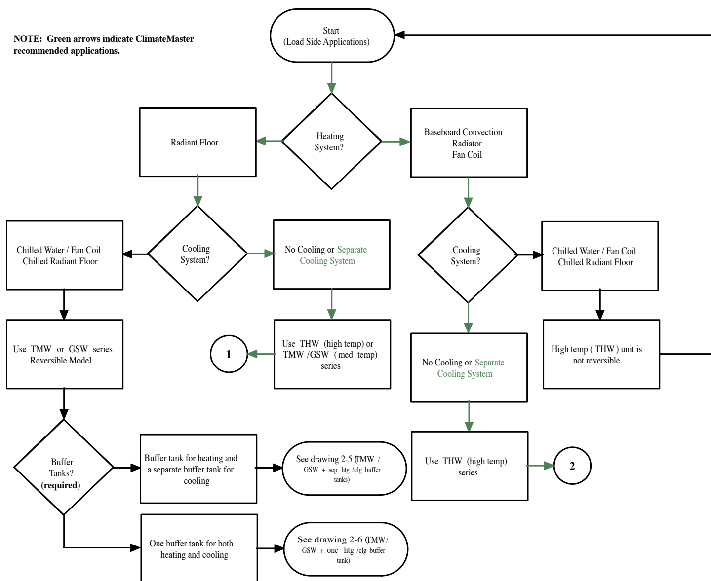
Figure 2-3a: System Selection Flow Chart (Part I)
