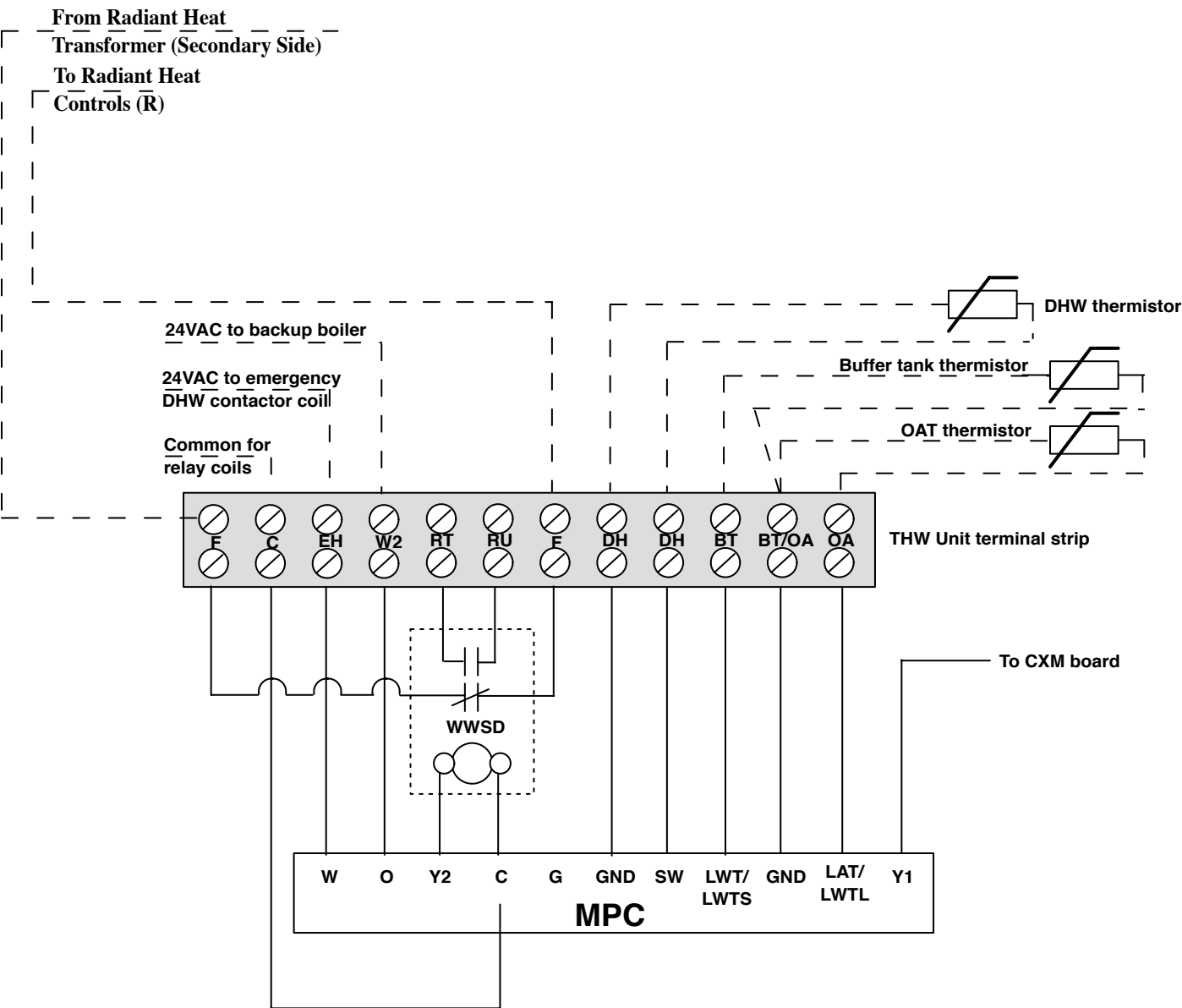
Drawing 4-1: THW Unit - Internal Pumps / No Cooling / Indirect DHW Tank
