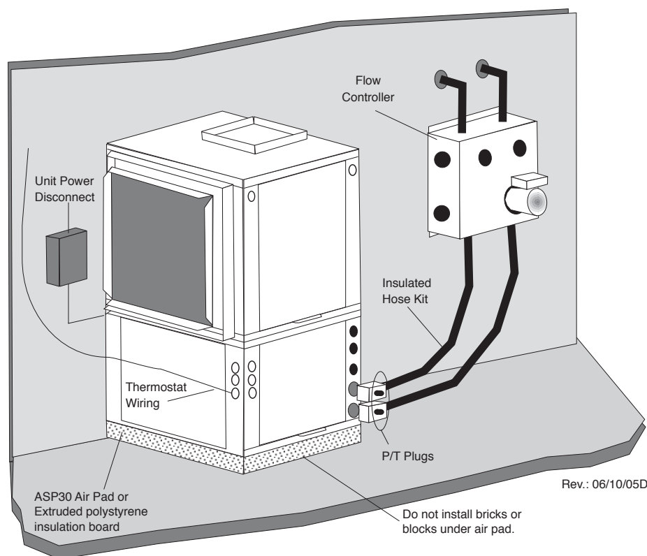
Figure 3-6: Typical Ground-Loop Application
