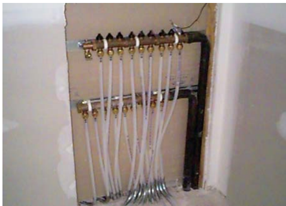
Figure 2-11: Radiant Floor Zone Manifold
