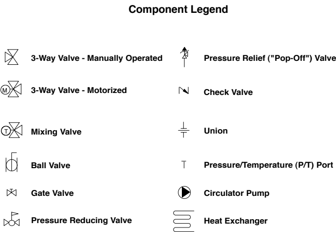
Figure 2-4: Component Legend for Drawings 2-1 to 2-9
