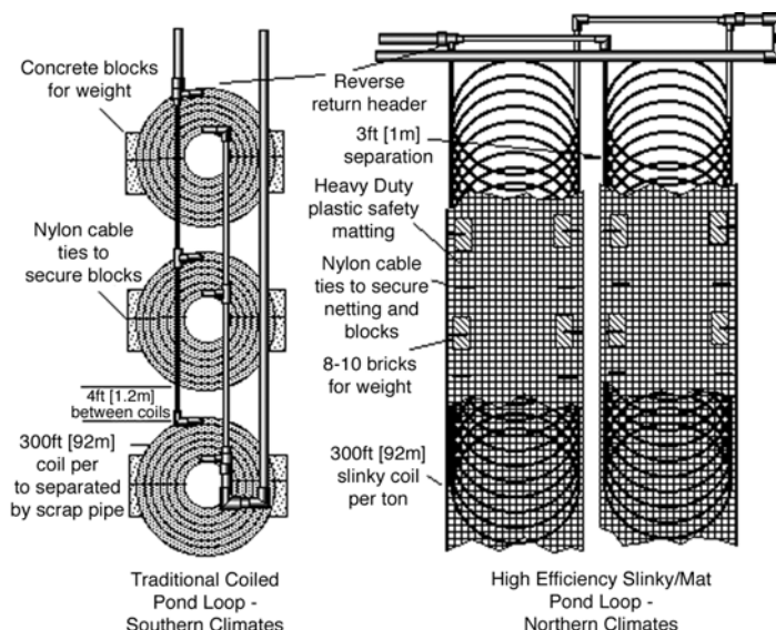
Figure 3-8: Typical Pond/Lake Loop Configurations
