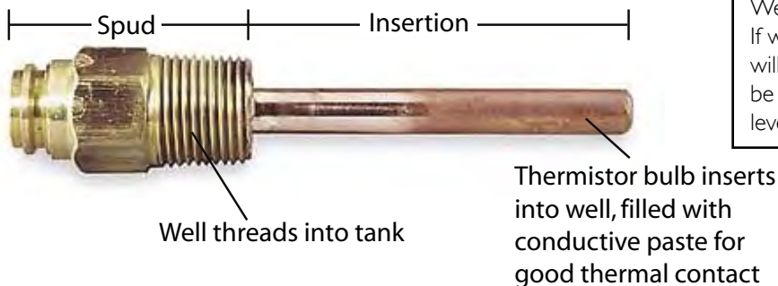
Figure 2-6: Well-Type Thermistors & Aqua-Stats
