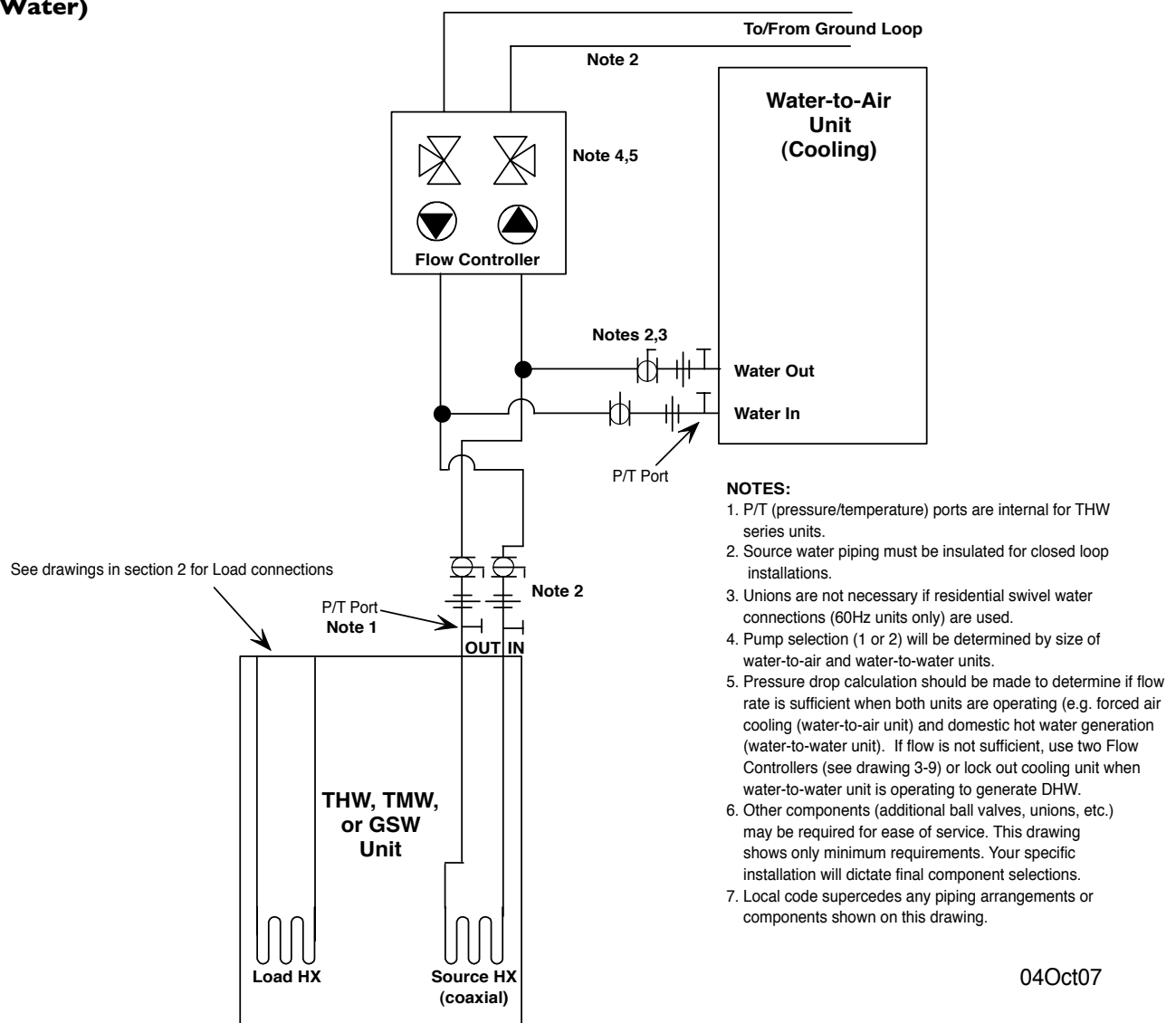
Drawing 3-4: Water-to-Water Source Piping - THW (No Source Pumps) or TMW / GSW Units - Water-to-Air Cooling (Shared Pumping with Water-to-Water)
