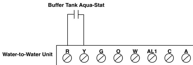
Drawing 4-6: TMW or GSW Unit - External Pumps* / No Cooling
