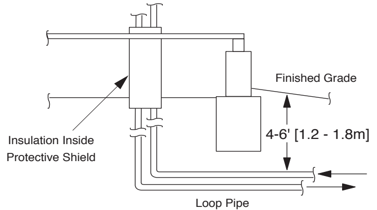
Figure 3-12: Pier and Beam (Craw Space) Detail
