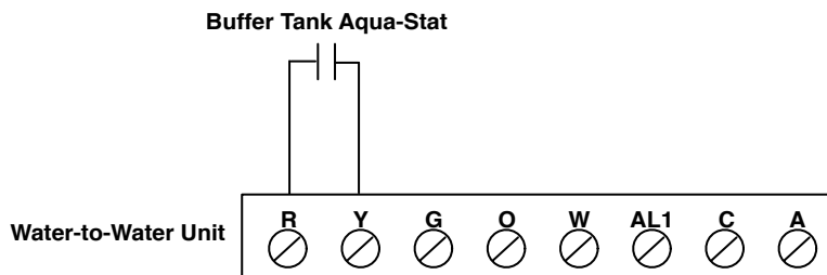
Drawing 4-7: TMW or GSW Unit - External Pumps* / Cooling with Separate Water-to-Air Unit
