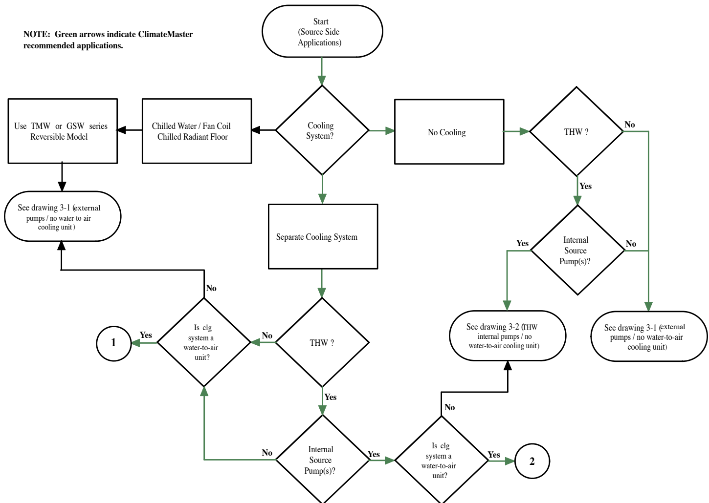
Figure 3-1a: System Selection Flow Chart (Part I)
