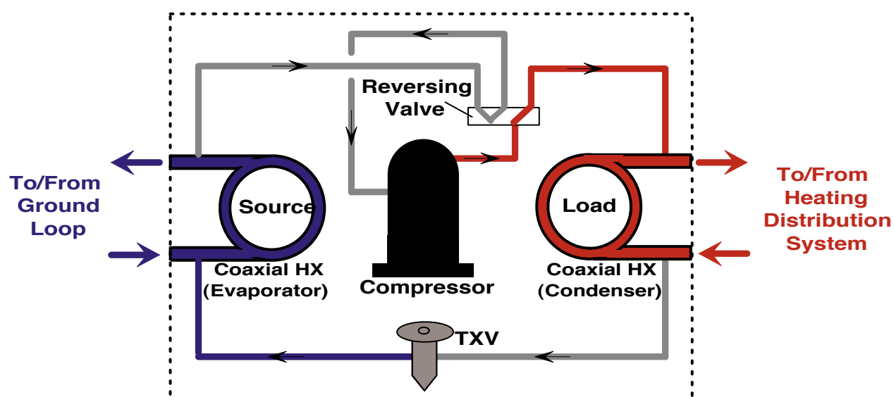
Figure I-3: Reversible Water-to-Water Heat Pump, Heating Mode
