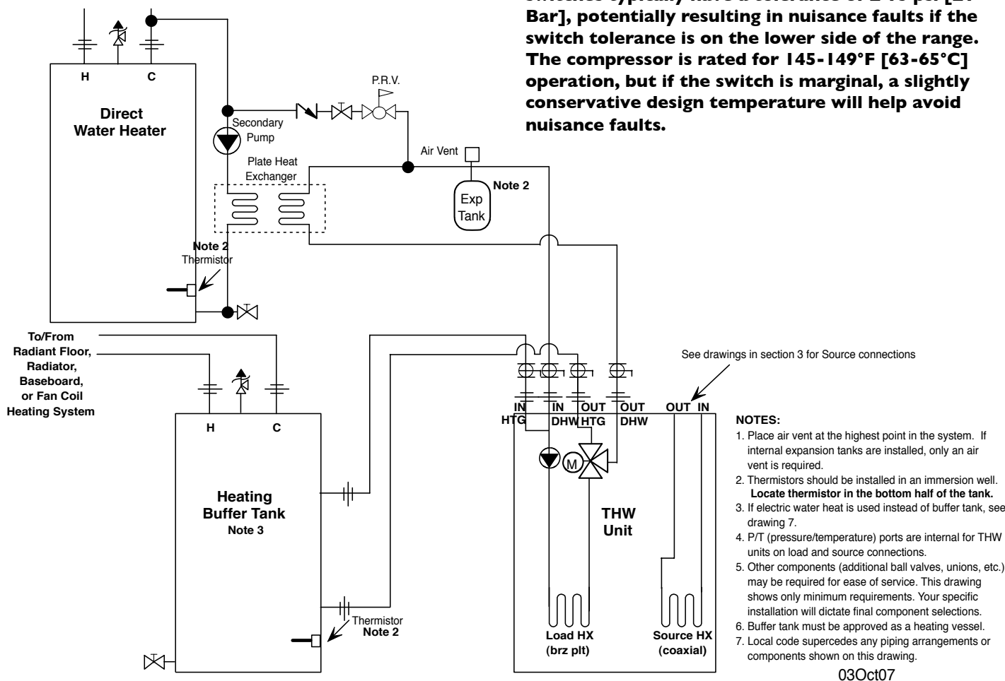
Drawing 2-2: THW Typical Load Piping - Water Heater with Secondary Heat Exchanger / No Cooling or Separate Cooling System
