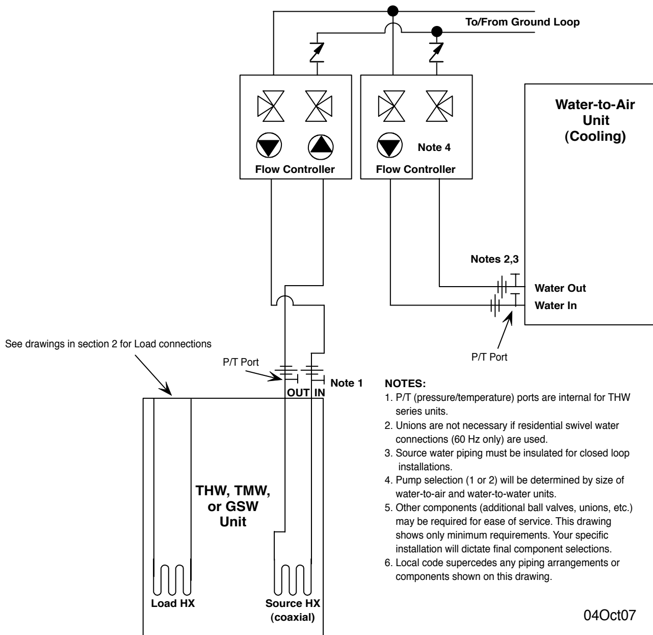
Drawing 3-3: Water-to-Water Source Piping - THW (No Source Pumps) or TMW / GSW Units - Water-to-Air Cooling with Separate Loop Pumps (ClimateMaster Preferred System When Cooling is Desired)
