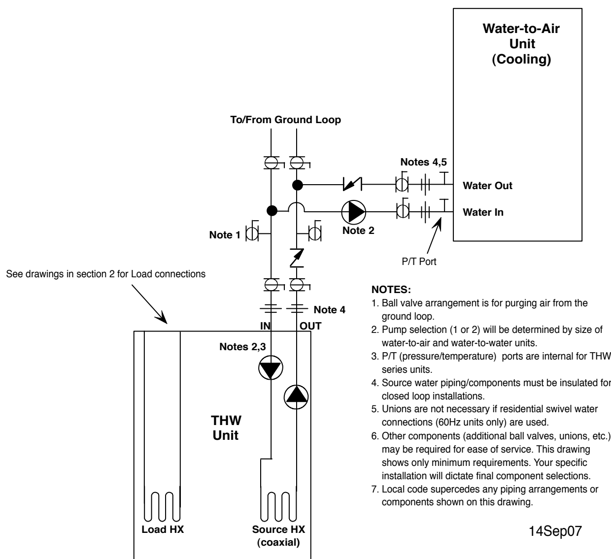
Drawing 3-5: THW Source Piping (Internal Source Pumps) - Separate Water-to-Air Cooling System
