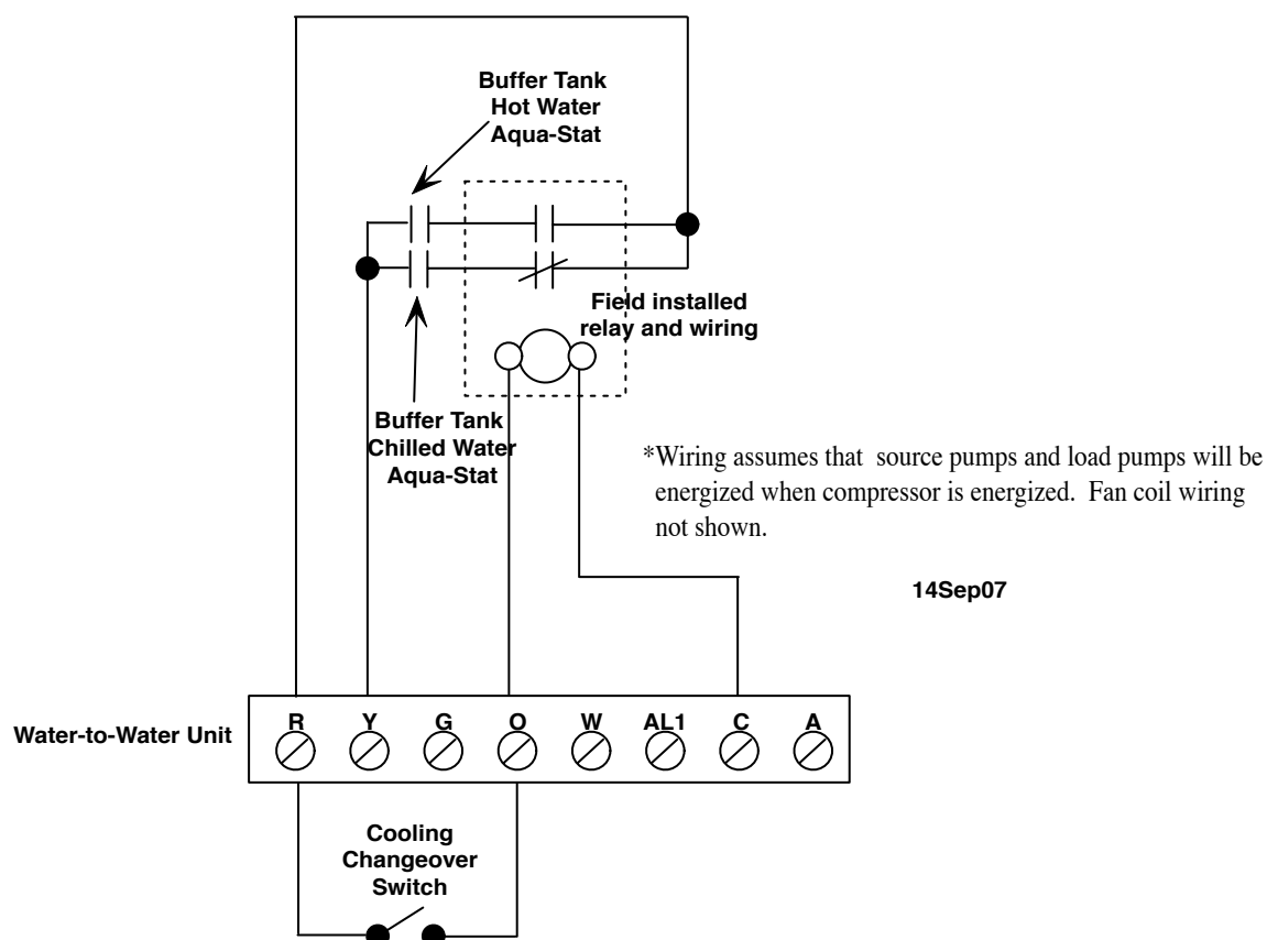
Drawing 4-9: TMW or GSW Unit - External Pumps* / Cooling with Chilled Water (Fan Coils)
