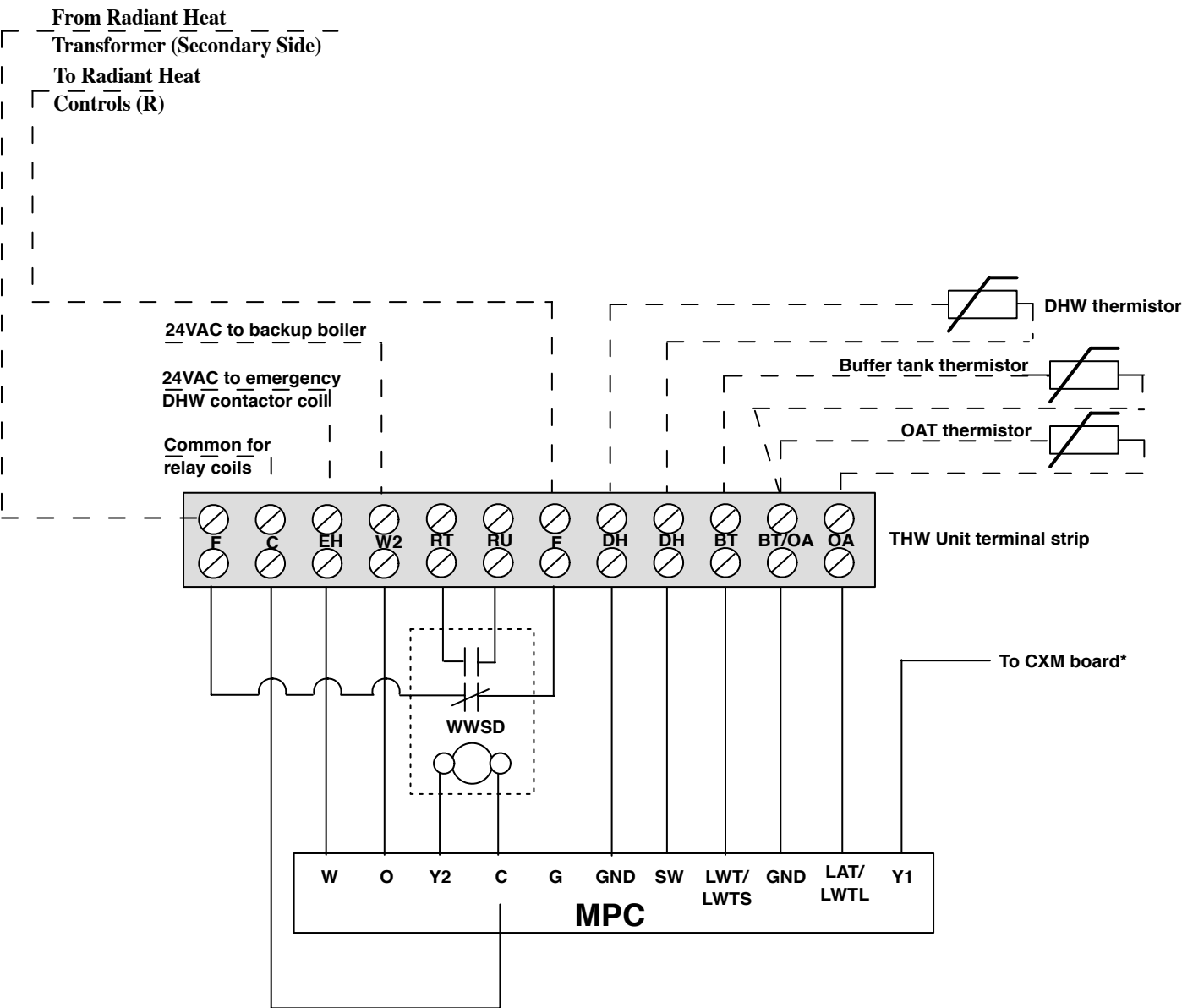
Drawing 4-3: THW Unit - External Pumps* / No Cooling / Indirect DHW Tank
