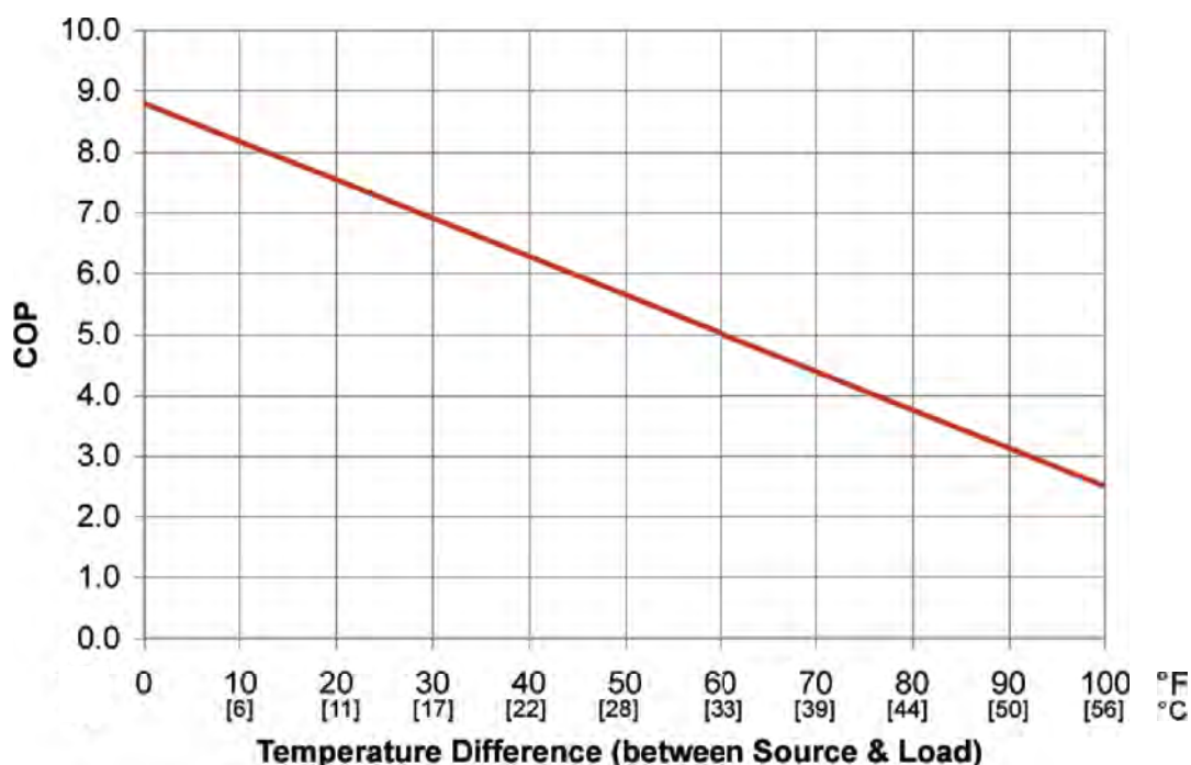
Figure 1-5: COP vs TD
