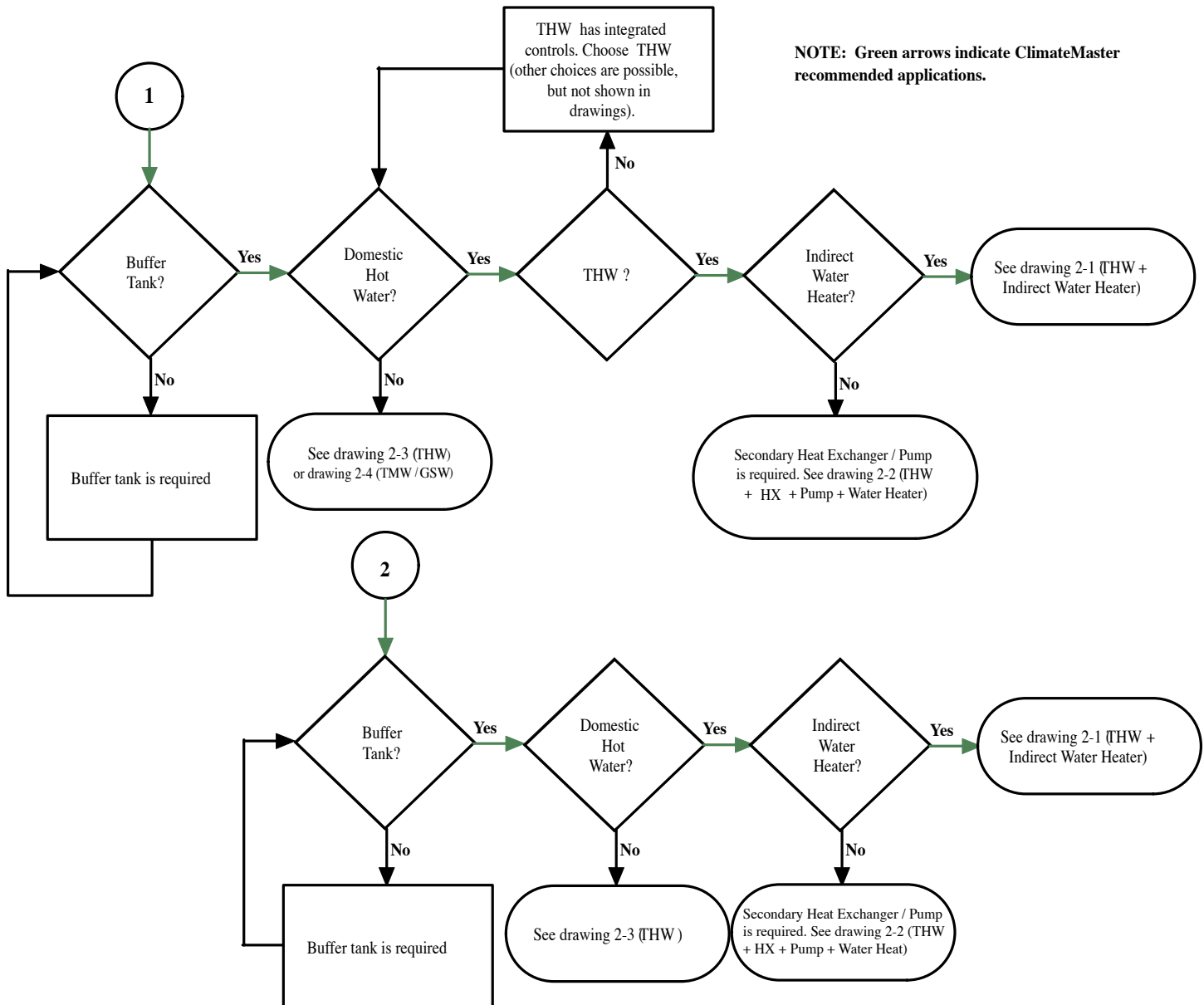
Figure 2-3b: System Selection Flow Chart (Part 2)
