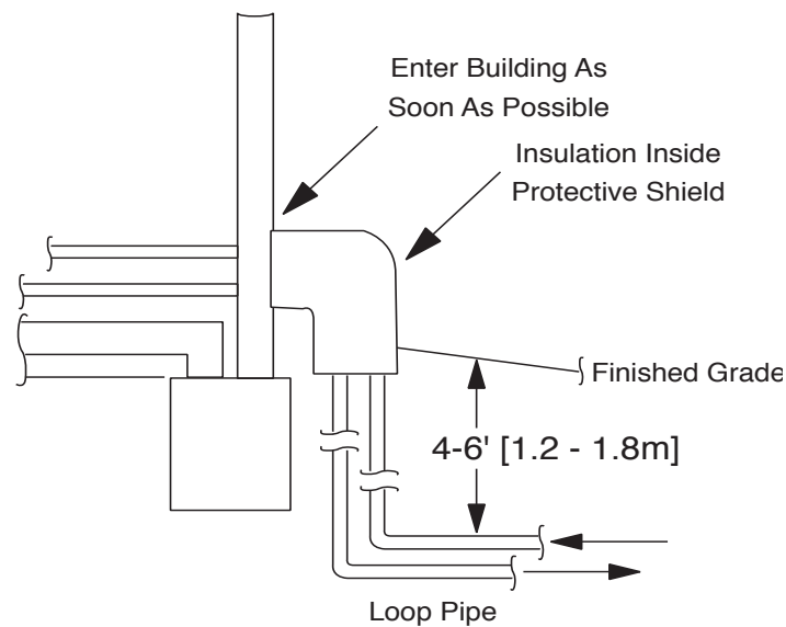
Figure 3-11: Retrofit Construction Detail
