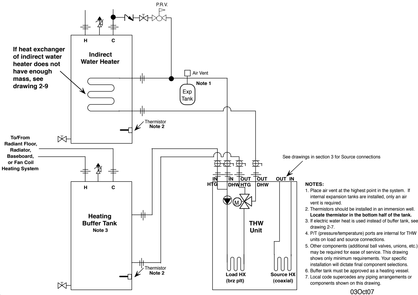
Drawing 2-1: THW Typical Load Piping - Indirect Water Heater / No Cooling or Separate Cooling System
