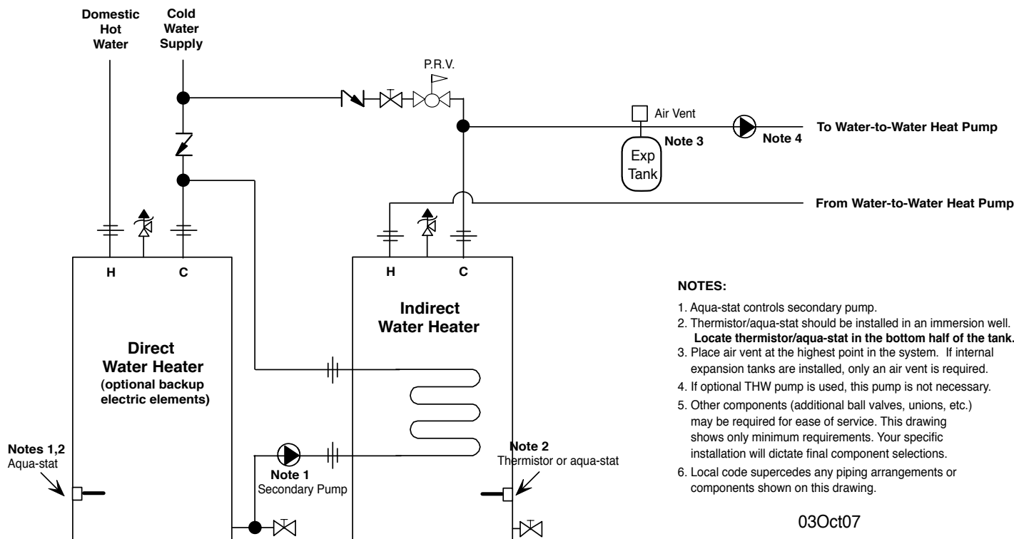
Drawing 2-9: Alternate DHW Piping - Indirect Water Heater with Low Mass Heat Exchanger
