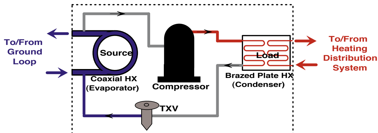
Figure I-3: Reversible Water-to-Water Heat Pump, Heating Mode
