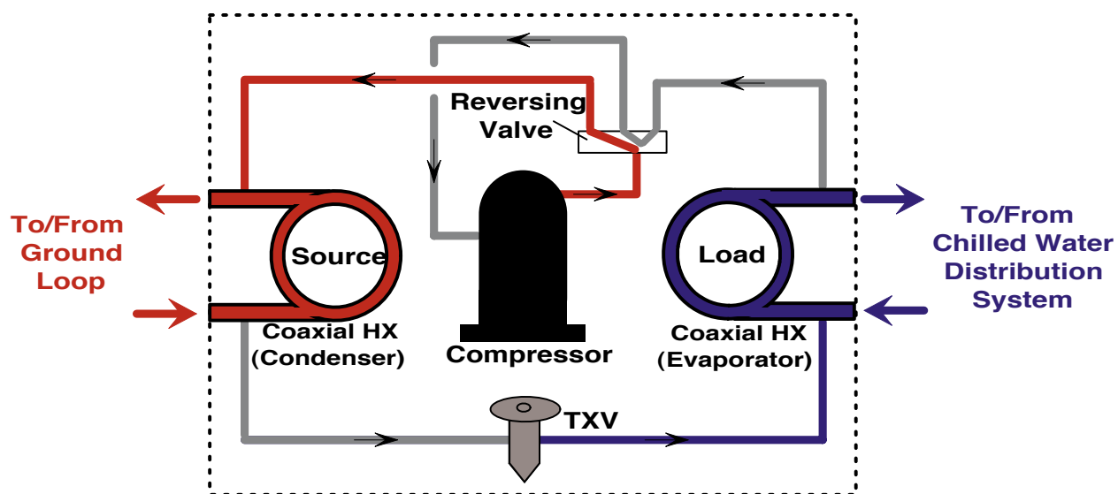
Figure I-4: Reversible Water-to-Water Heat Pump, Cooling Mode
