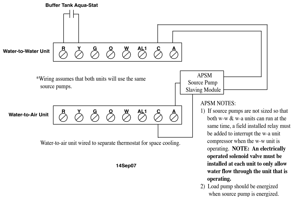
Drawing 4-8: TMW or GSW Unit - External Pumps* / Cooling with Separate Water-to-Air Unit
