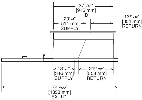
Illustration ST-A1291-44-00
