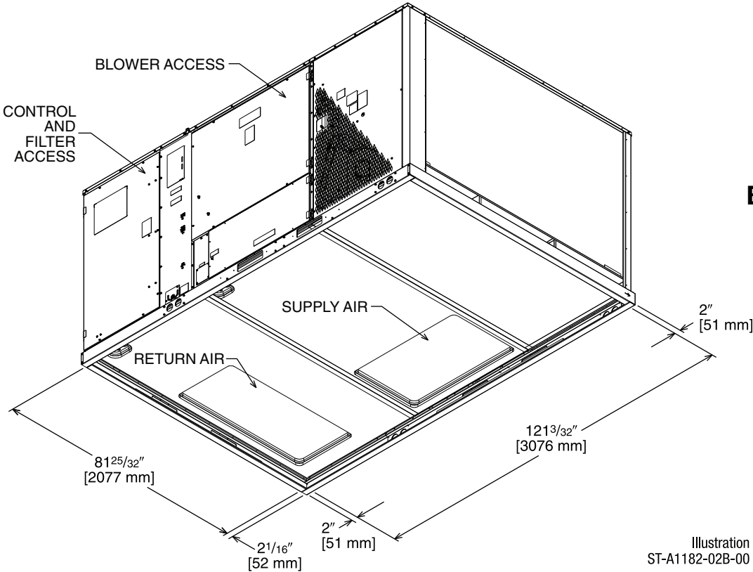
BOTTOM VIEW
