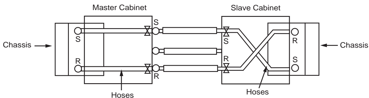
Option 2 - Field supplied and brazed piping to be straight across. Mark shutoffs inside slave cabinet. Cross hoses to chassis.
