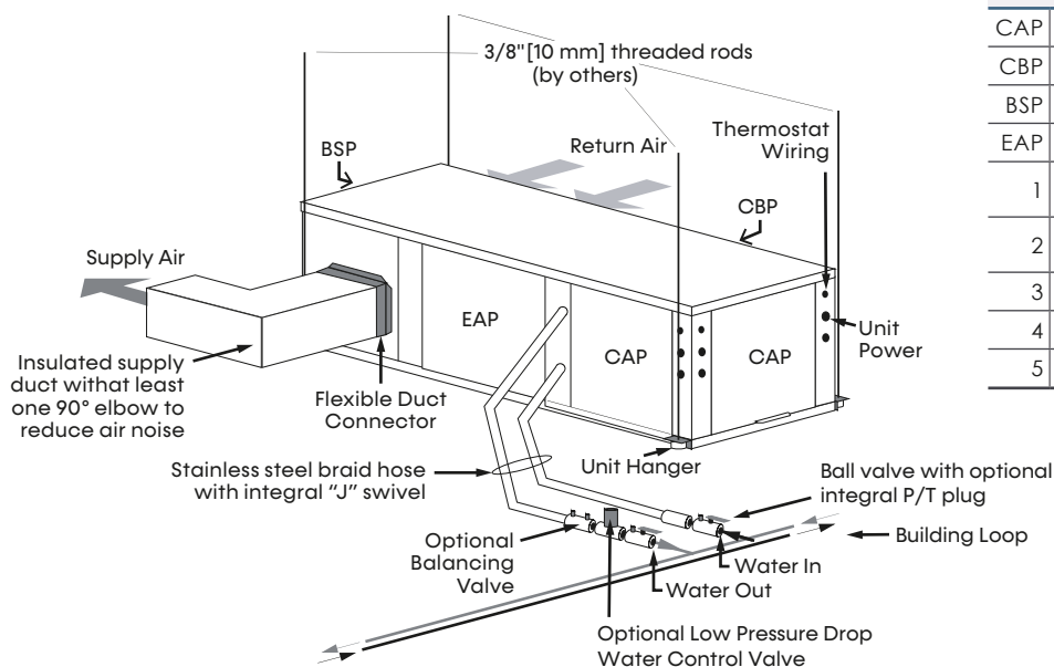
Figure 2: Typical Unit Installation
