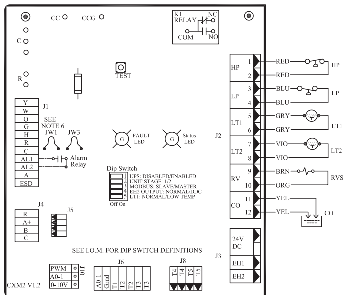
Figure 9: LT1 Limit Setting
