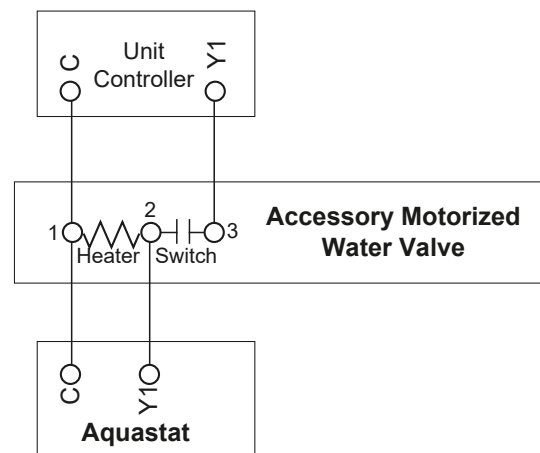
Figure 12: Optional Motorized Water Valve Wiring
