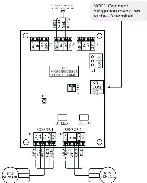
Figure 13: RDS Board
