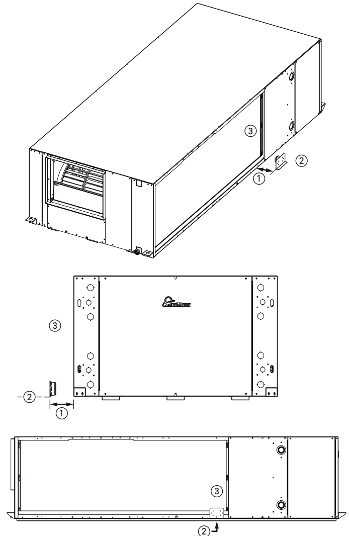
Figure 14: Sensor Placement
