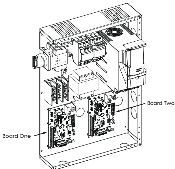
Figure 10: SB Horizontal Control Box (Representative)
