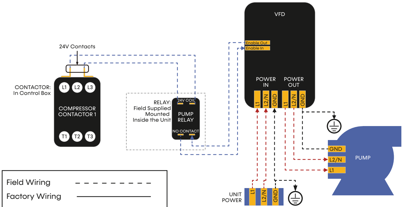
Figure 17: External Pump Control with VFD Diagram
