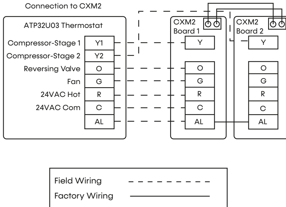
Figure 15: Thermostat Connection
