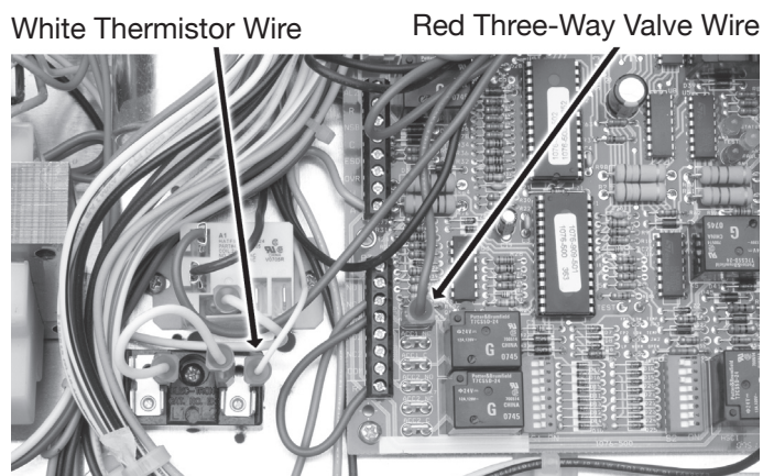
Figure 2. Normal Unit Wiring
