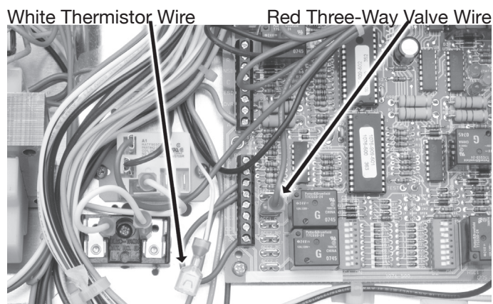
Figure 1. Flushing/Purging Wiring
