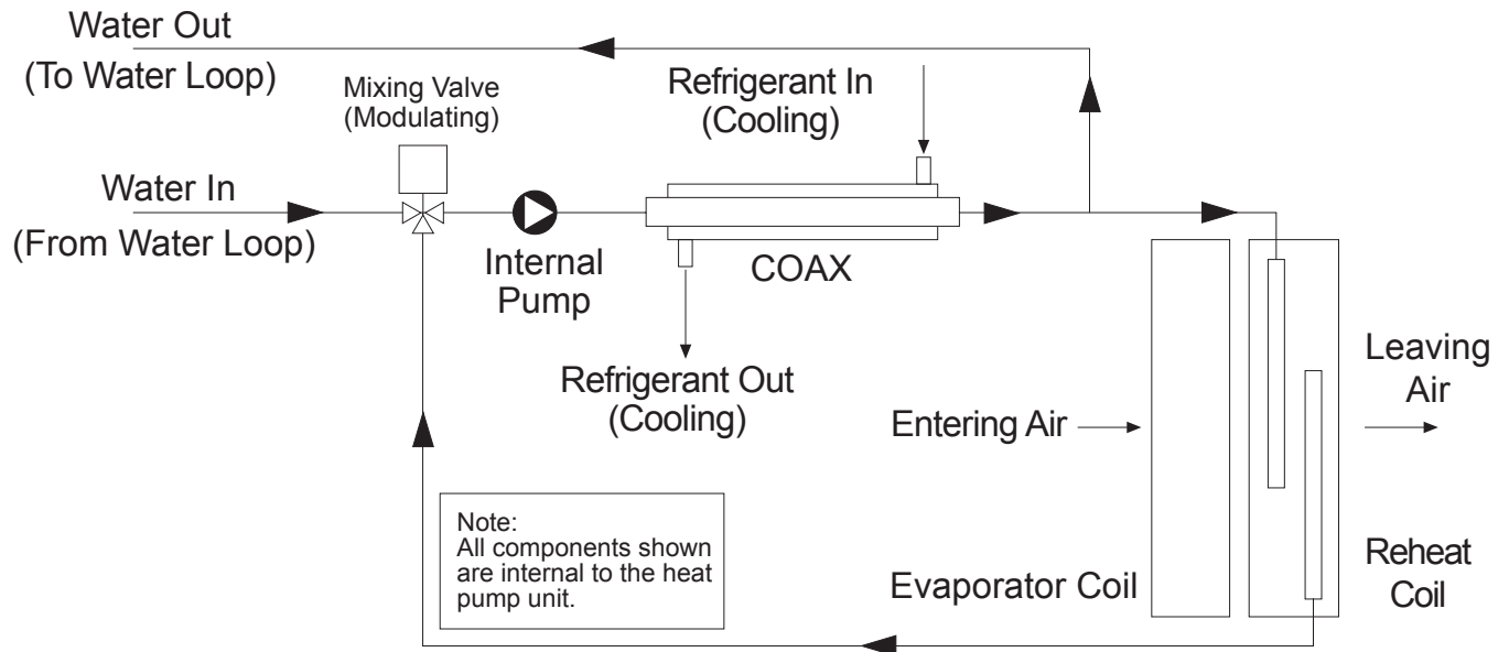
Figure 2: ClimaDry® Schematic
