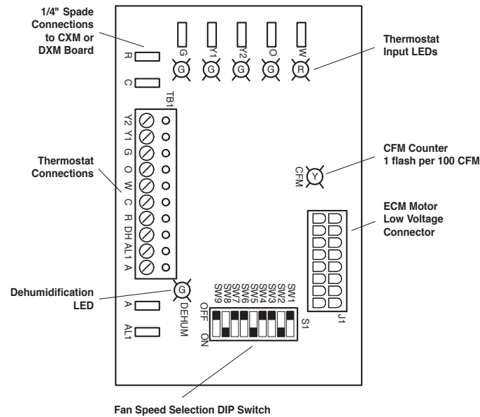
Figure 26a: ECM Version II Interface Layout
