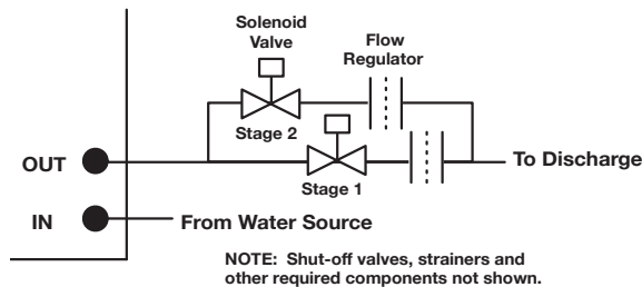
Figure 24: Two-Stage Piping
