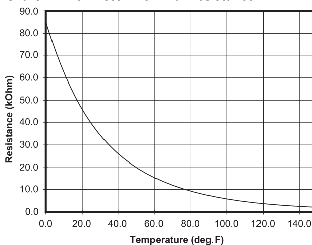
Chart 1: Thermistor Nominal Resistance
