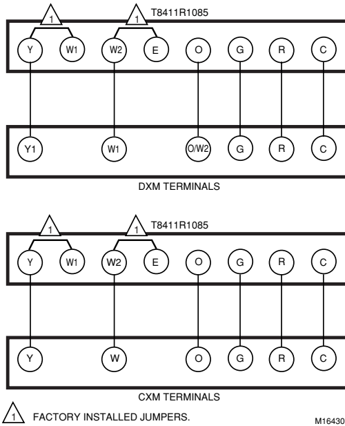
Fig. 5. DXM and CXM terminal wiring diagrams.
