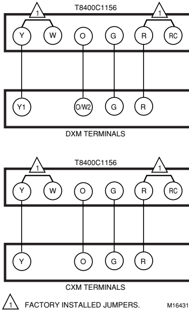
Fig. 5. DXM and CXM terminal wiring diagrams.
